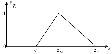
Figure 2 – A triangular membership function
