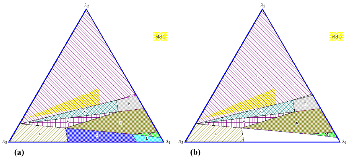
Figure 4 – Fuzzy analysis of the objective function coefficients using indifference regions ( \gamma=0.0500_R )
