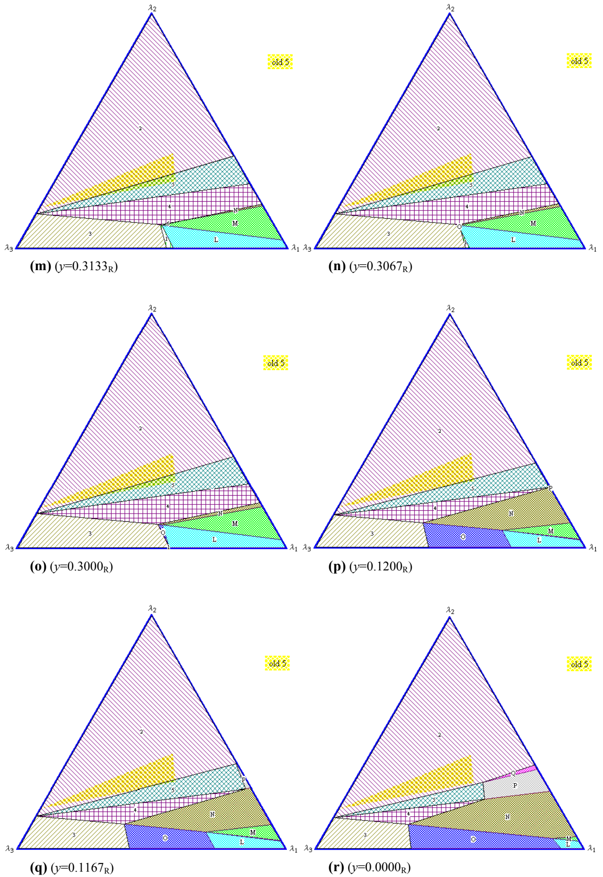
Figure 5 – Fuzzy analysis of the objective function coefficients using indifference regions
