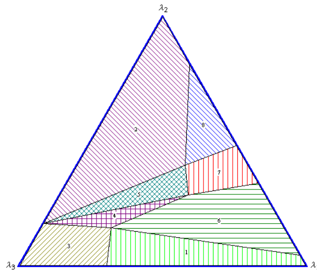
Figure 3 – Indifference regions corresponding to the initial basic efficient solutions
