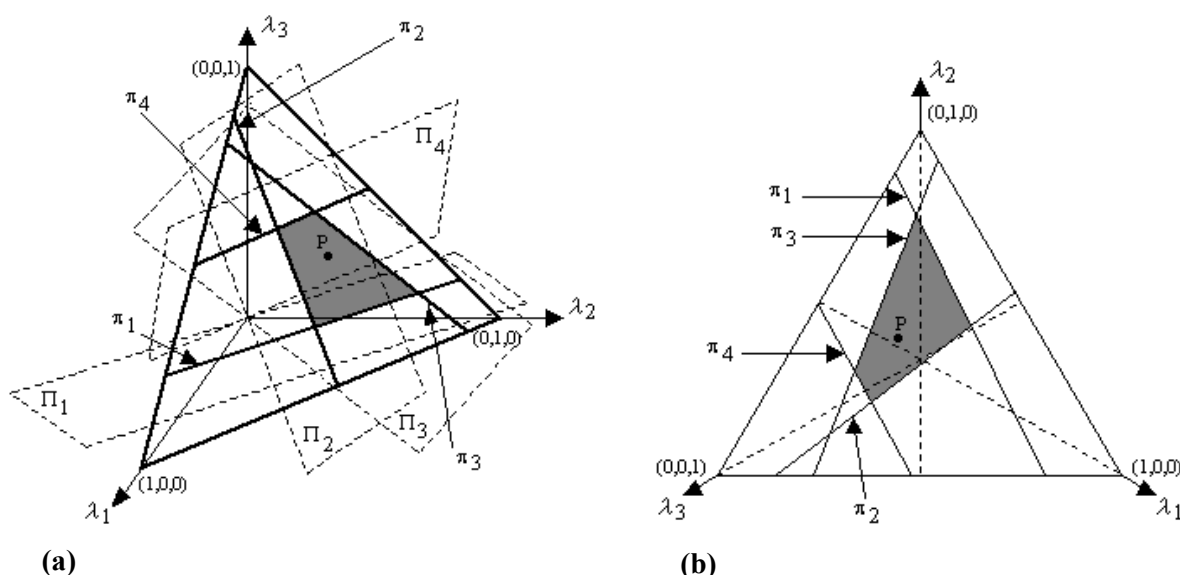
Figure 1 – Decomposition of \Lambda into indifference regions
