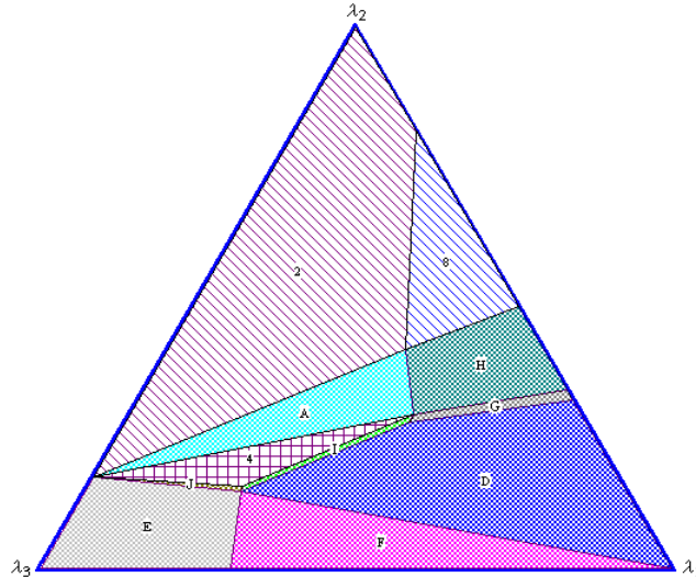
Figure 6 – Fuzzy analysis of RHS coefficients using indifference regions ( t=0.3367_R )
